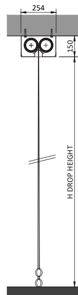
SECTION TYPE AT-H-E
